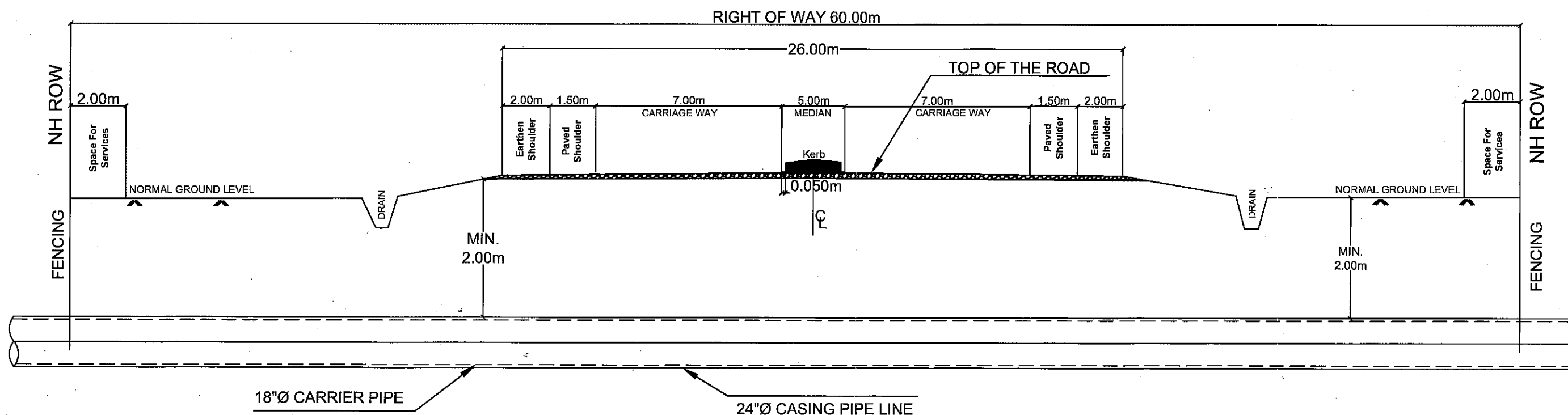
TYPICAL CROSS SECTION @ KM 126.350
