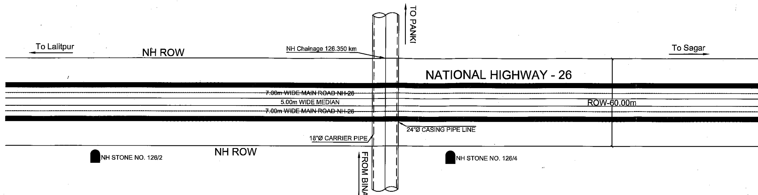
TYPICAL LAYOUT PLAN
